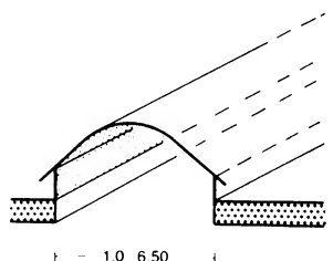
⑥ Continuous barrel skylight
